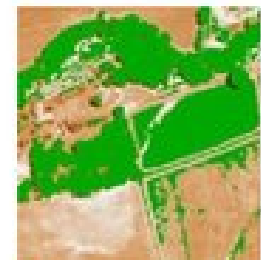
Soil Brightness Map
