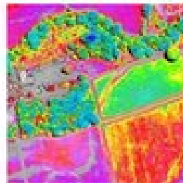
Sharp Vegetation Index
