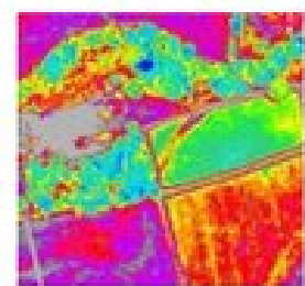
Green Vegetation Index
